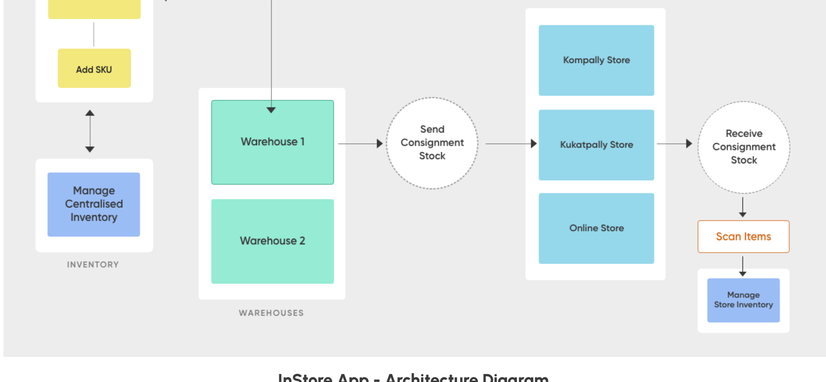
InStore App - Architecture Diagram
